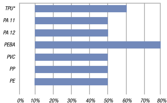
Typical Loading Levels for Bismuth Subcarbonate in Medical Polymers
